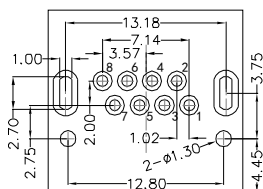
RECOMMENDED PCB LAYOUT VIEWED FROM COMPONENT SIDE
