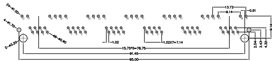
RECOMMENDED PCB LAYOUT VIEWED FROM COMPONENT SIDE
