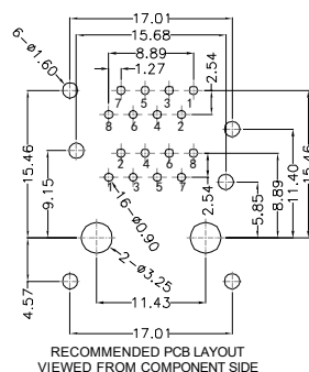
RECOMMENDED PCB LAYOUT VIEWED FROM COMPONENT SIDE
