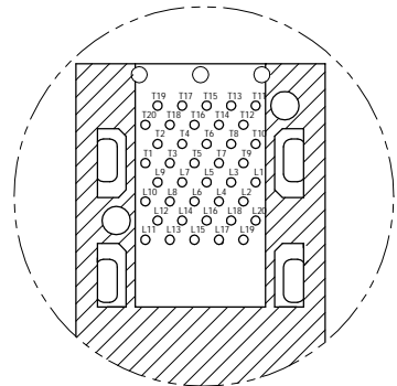
CONNECTOR PIN-OUT COMPONENT SIDE OF BOARD
