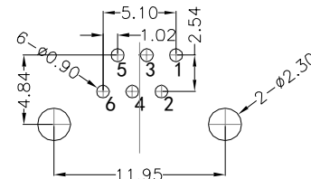
RECOMMENDED PCB LAYOUT VIEWED FROM COMPONENT SIDE
