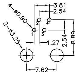
RECOMMENDED PCB LAYOUT VIEWED FROM COMPONENT SIDE
